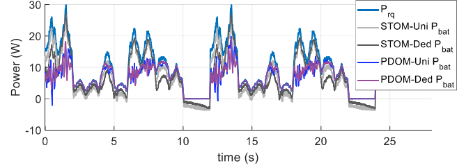
Fig. 11. Power scheduling simulation results with power supply and demand including noises.
