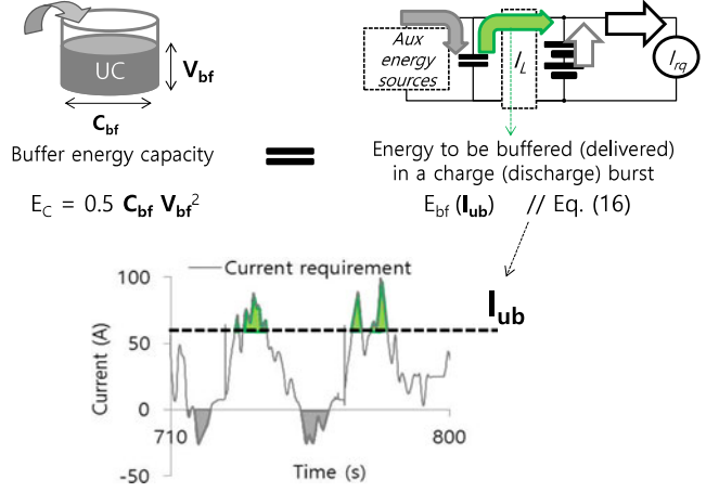
Fig. 6. Determination of current bounds for peak power reduction.
