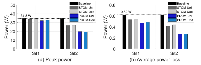
Fig. 10. Peak power (a) and average power loss (b) under Sit1 and Sit2.
