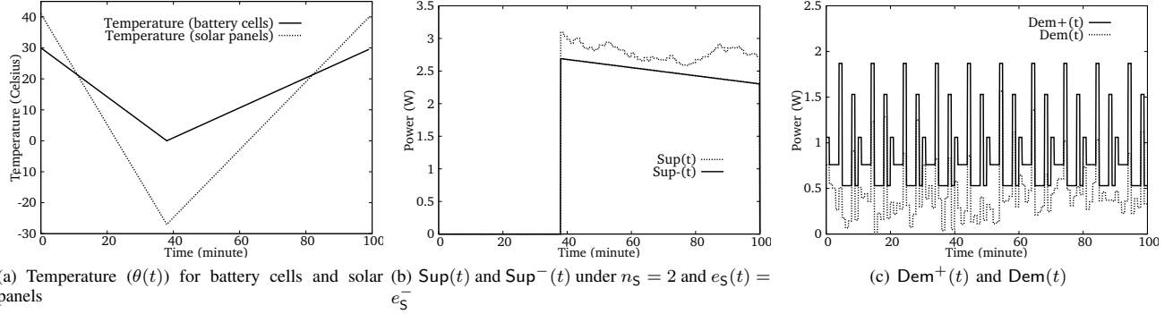
Fig. 6. Profiles of temperature, power supply from solar panels and power demand from sub-systems
